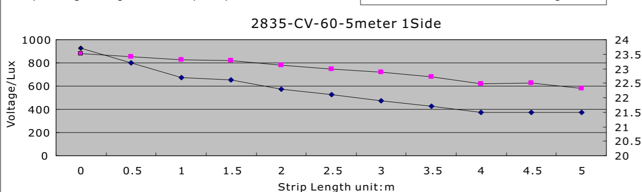
Strip Voltage & Brightness Drop Graph
