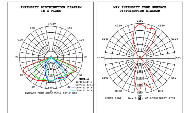
Luminous Intensity Distribution Diagram
