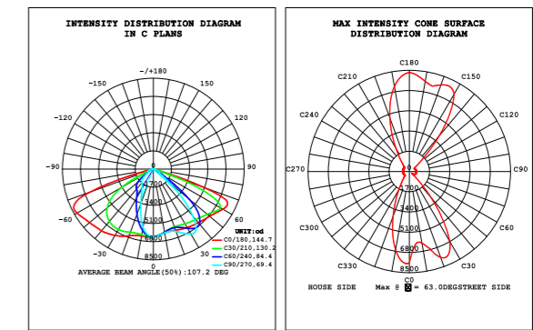
Luminous Intensity Distribution Diagram
