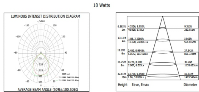
Luminous Intensity Distribution Diagram
