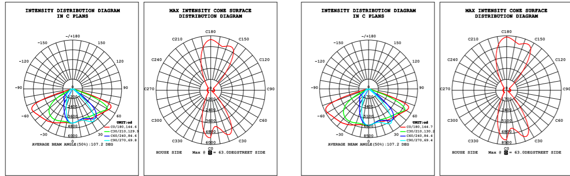
Luminous Intensity Distribution Diagram
