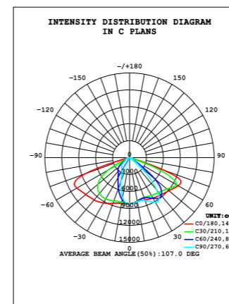
Luminous Intensity Distribution Diagram
