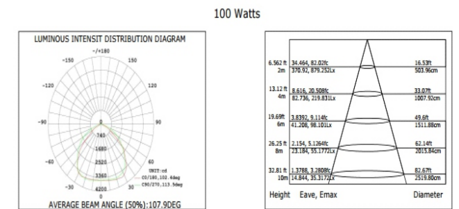
Luminous Intensity Distribution Diagram
