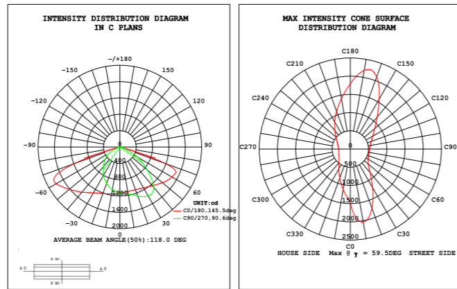
Luminous Intensity Distribution Diagram
