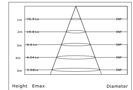
22 Watts Cornlight Diagram
