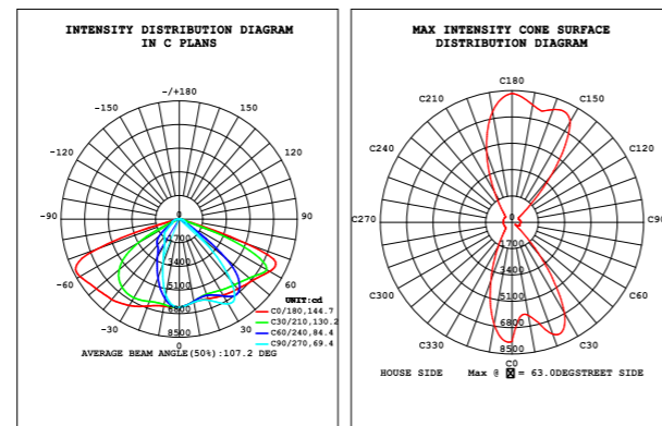
Luminous Intensity Distribution Diagram
