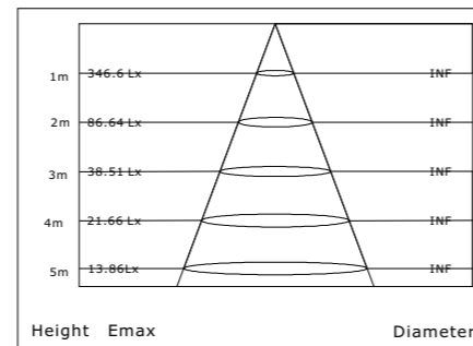
88 Watts Cornlight Diagram
