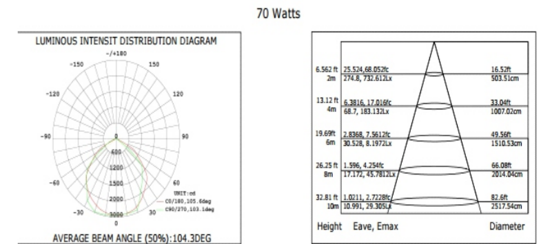
Luminous Intensity Distribution Diagram
